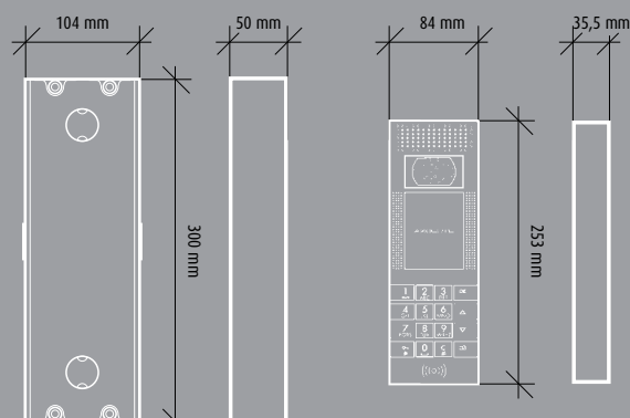
Flush mounted box
