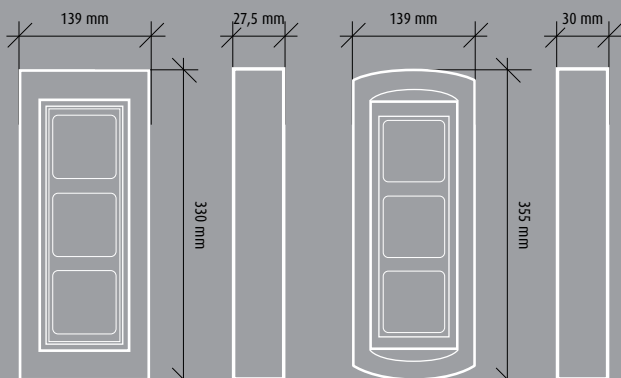
Steel frame + supporting frame Projection from wall: 11 mm
